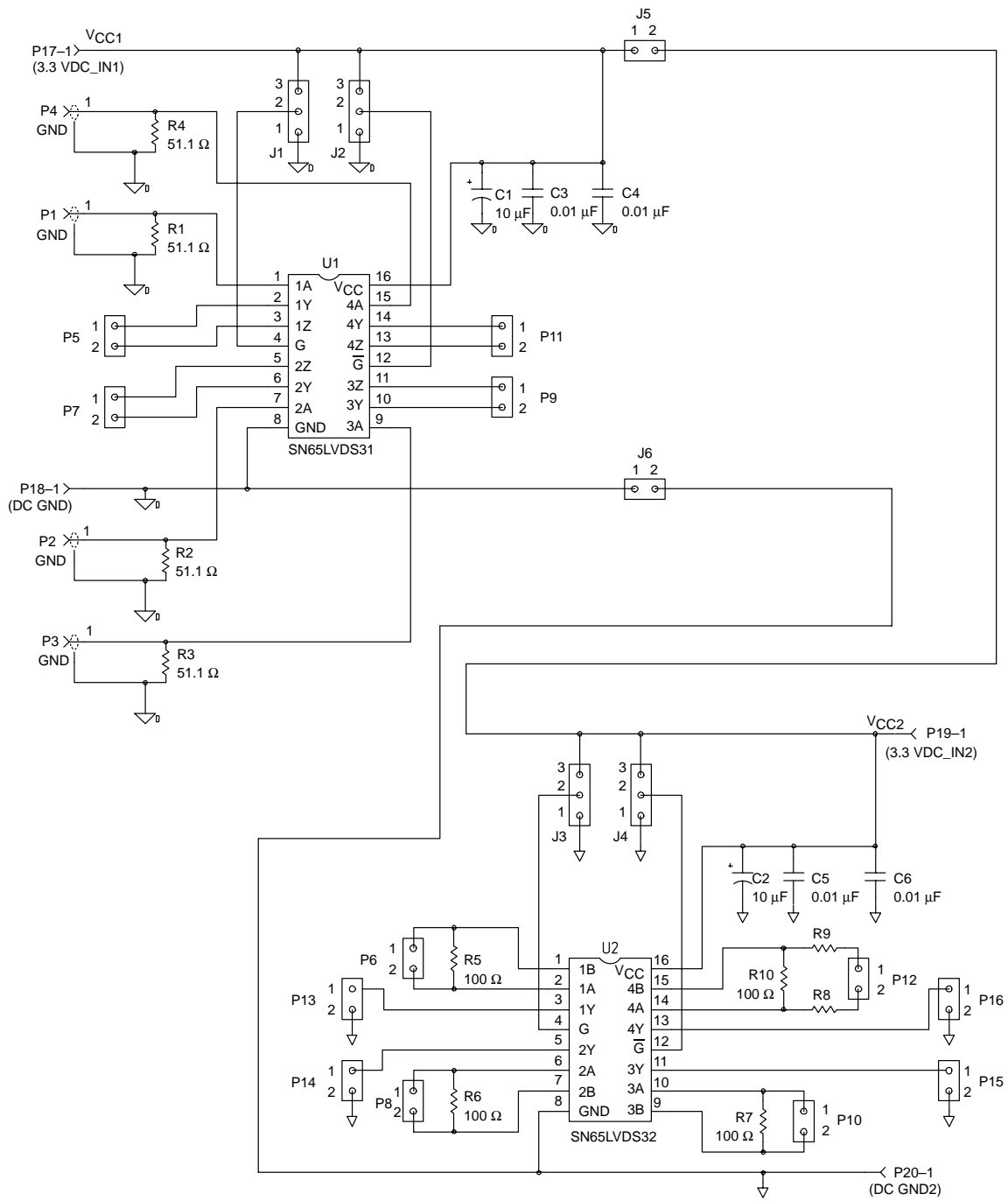
Figure 2–1. The EVM Schematic Diagram
